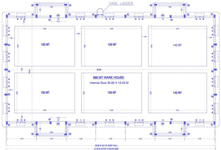
890 MT WARE HOUSE UNIT PLAN
